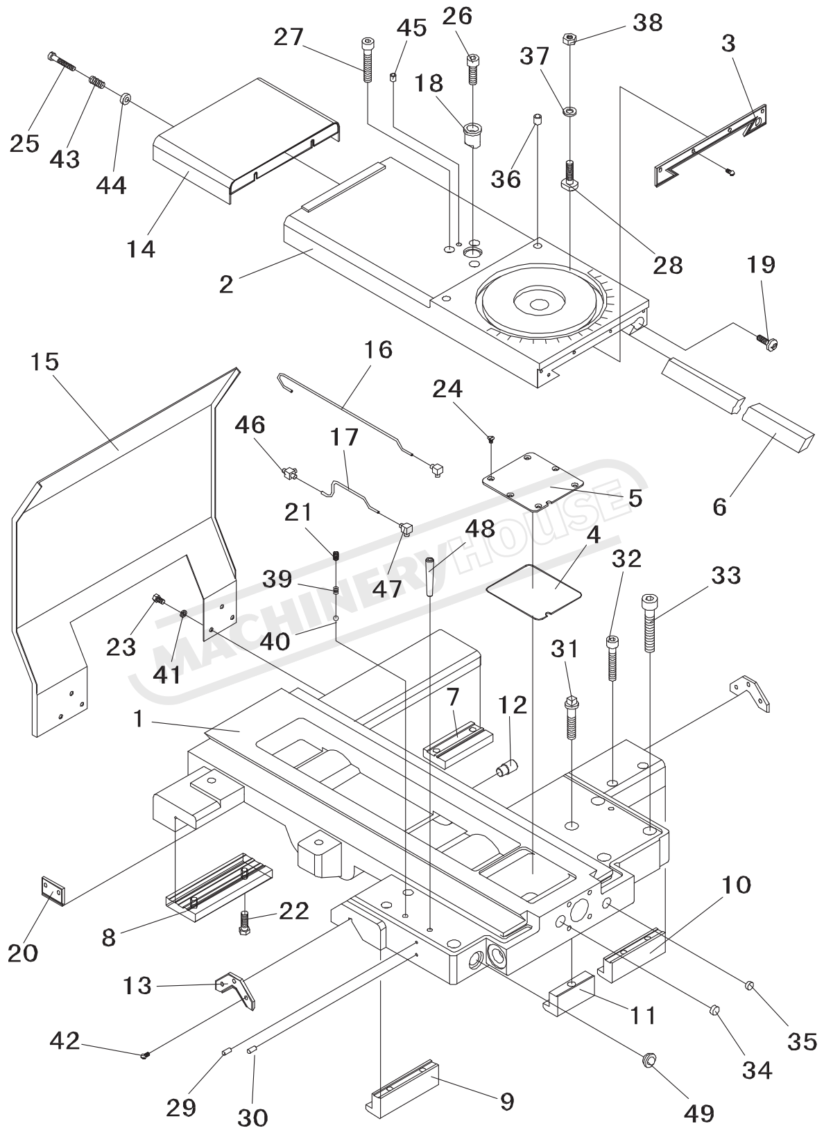
图05-01 刀架及床鞍 FIG05-01 SLIDE AND SADDLE
